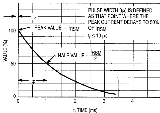
Figure 5. Pulse Waveform
