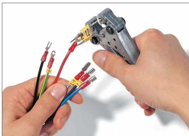
The sleeve applicator tool allows markers to be fitted after crimping.
