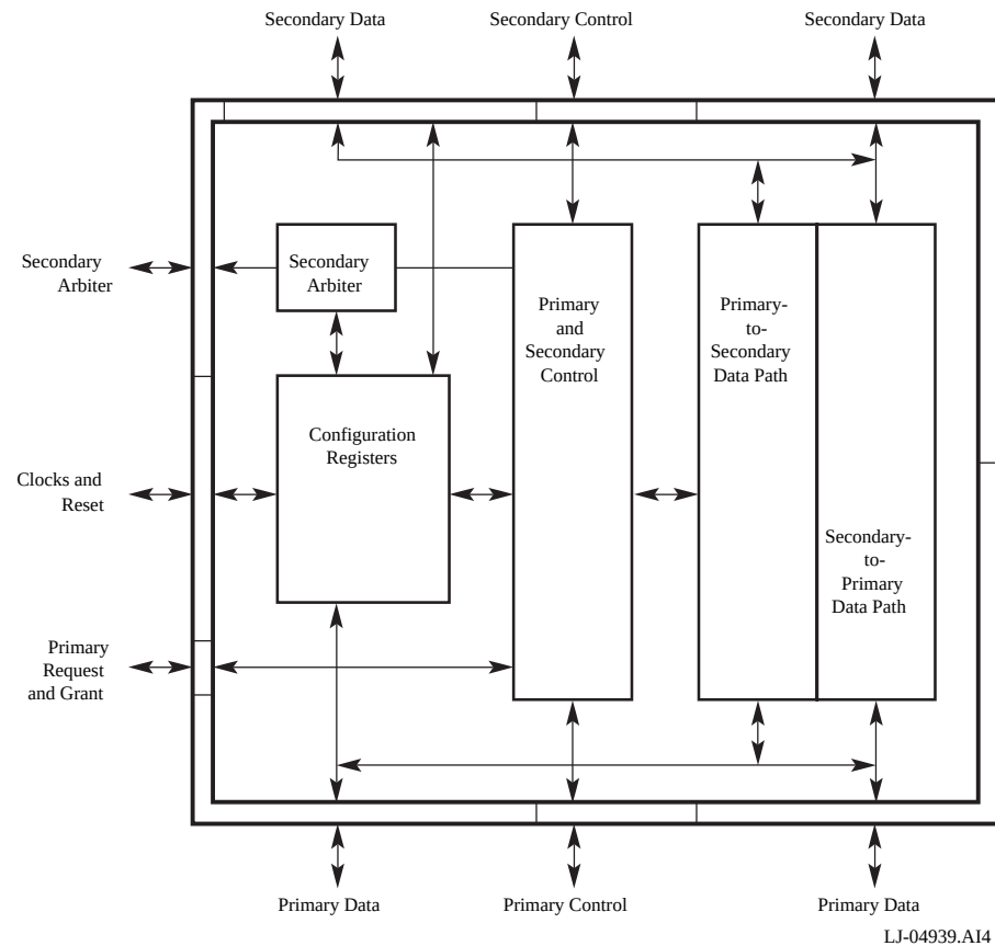
Figure 3. 21152 Block Diagram
