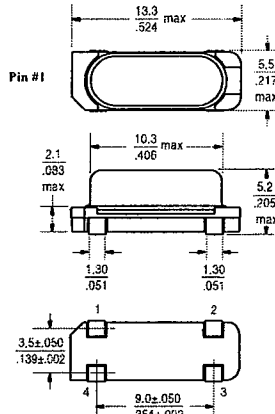
49SNC package
