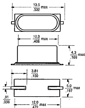
49SMLB package
