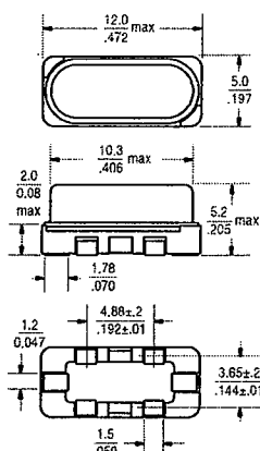
49SAB/SUB package
