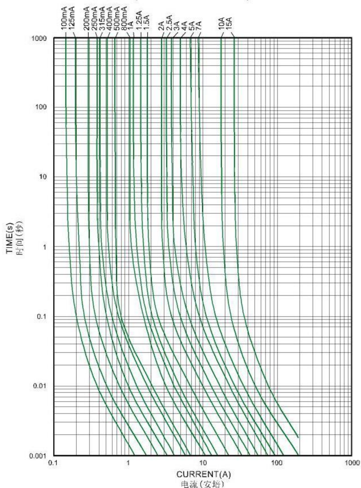
20N 平均 I-T 曲线图 (仅供参考) 20N AVERAGE I-T CHARACTERISTICS CURVE (FOR REFERENCE)
