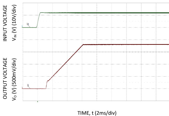
Figure 18. Typical Start-up Using Input Voltage ( V_{IN}=12\text{V} , I_o=I_{o,max} ).
