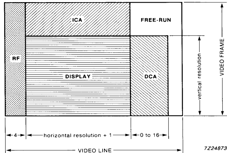
Fig.5 DRAM Timing Windows.
