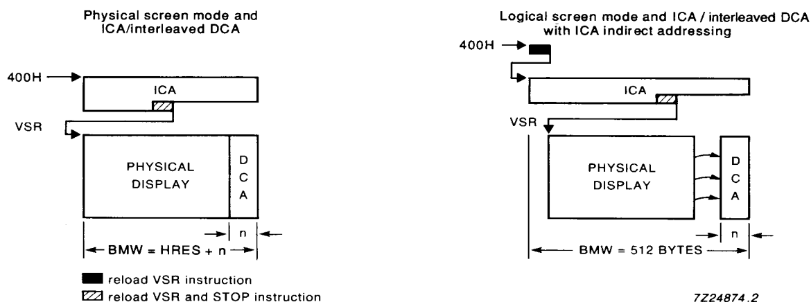
Fig.10 ICA/interleaved DCA and Physical display.
