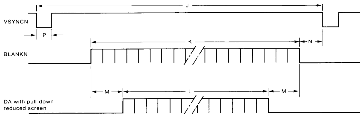
Fig.14 Vertical synchronization timing.
