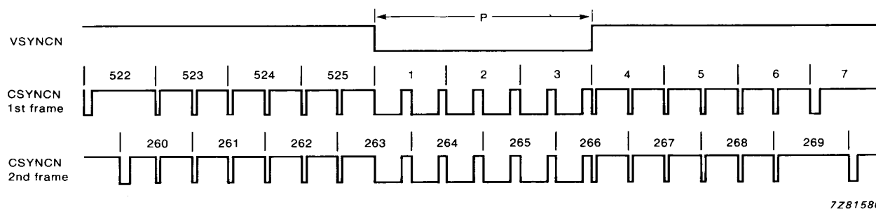
Fig.16 CSYNCN timing in the 60 Hz, interlace or interlace field repeat mode.
