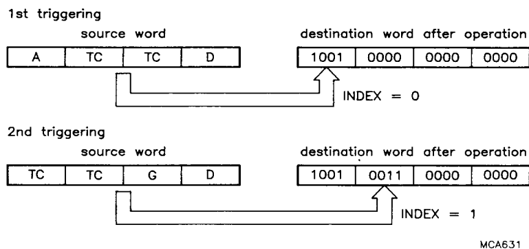
Fig.31 COMPACT example in 4 bits/pixel.
