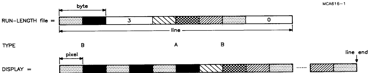
Fig.24 Run-length file display, 4 bits/pixel.
