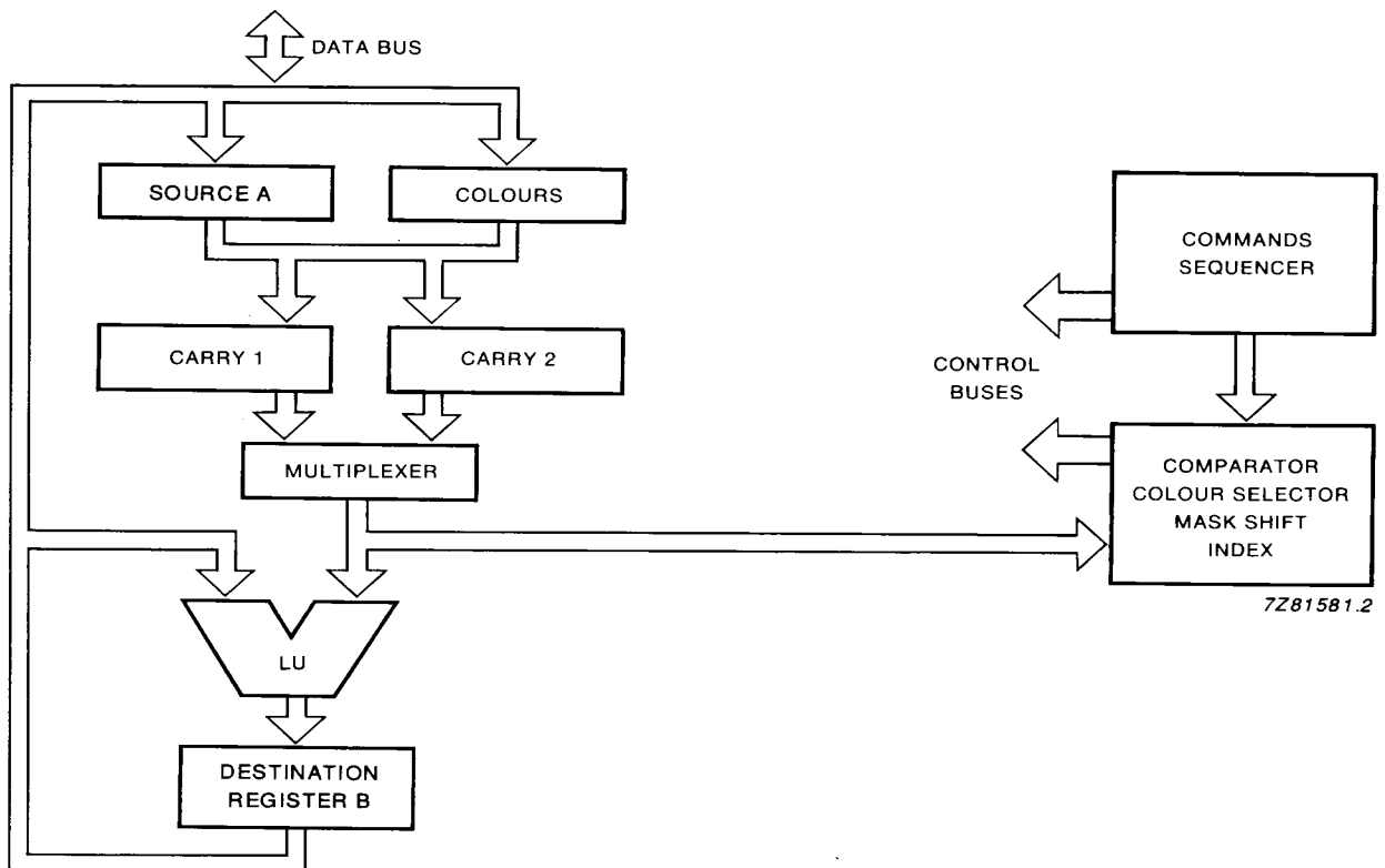
Fig.27 PIXAC block diagram.
