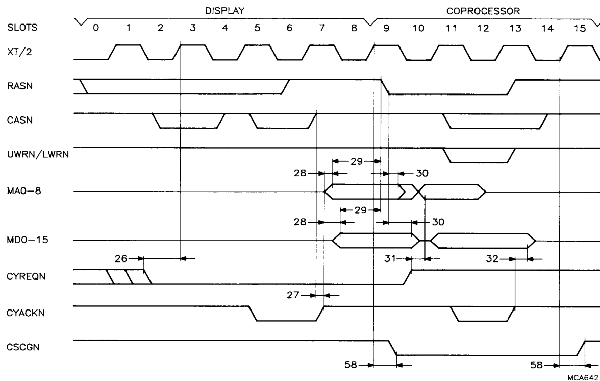
Fig.47 Coprocessor &lt;-&gt; memory or register access in FAST mode.
