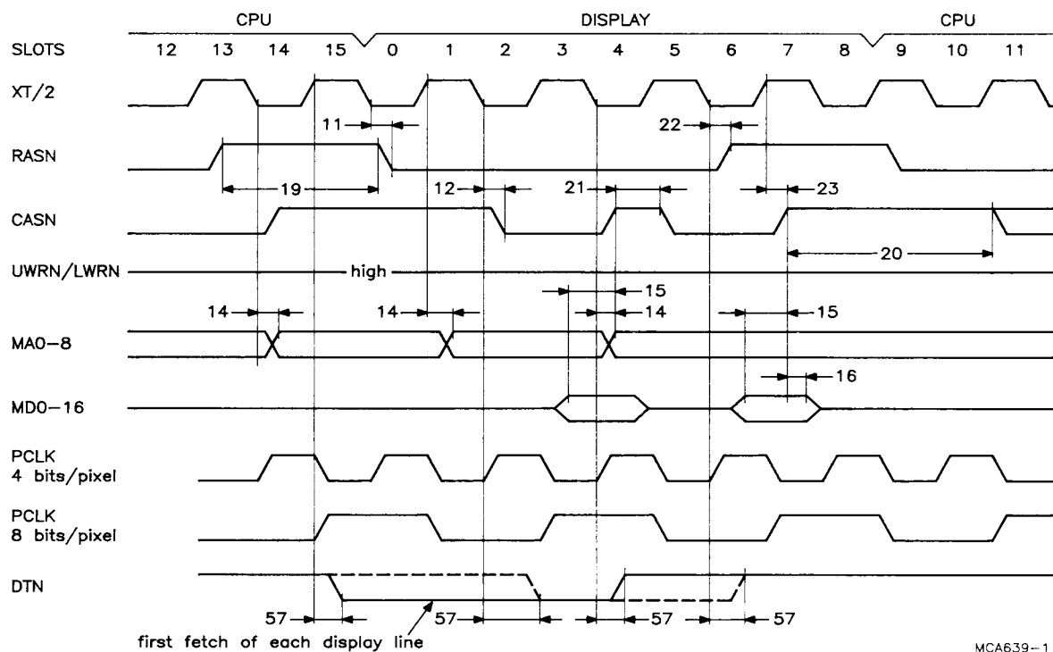
Fig.44 Display cycle in FAST mode.
