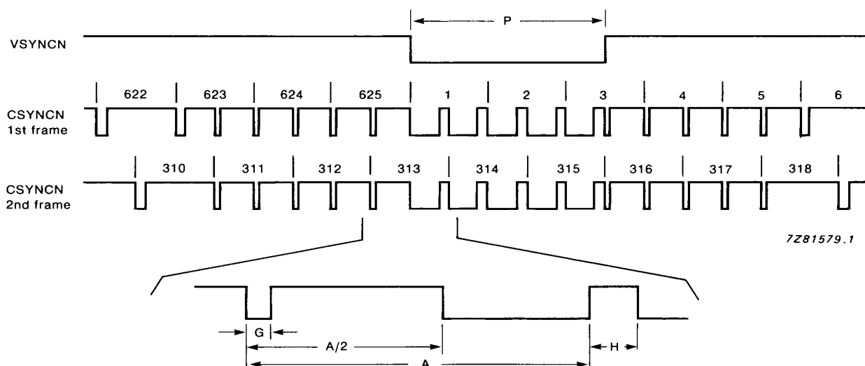
Fig.15 CSYNCN timing in the 50 Hz, interlace or interlace field repeat mode.
