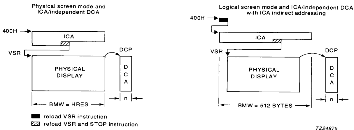
Fig.11 ICA/independent DCA and Physical display.
