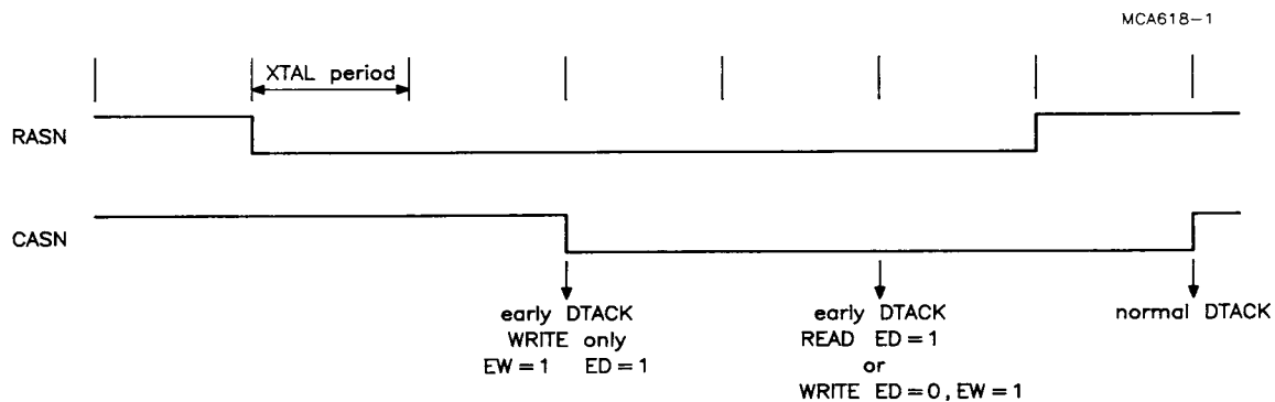
Fig.4 DTACK assertion in SLOW mode timing.
