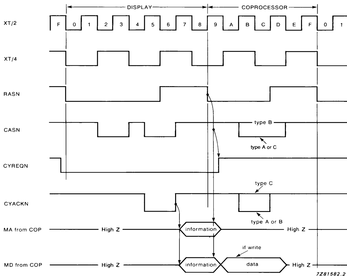
Fig.34 Coprocessor interface in FAST mode.
