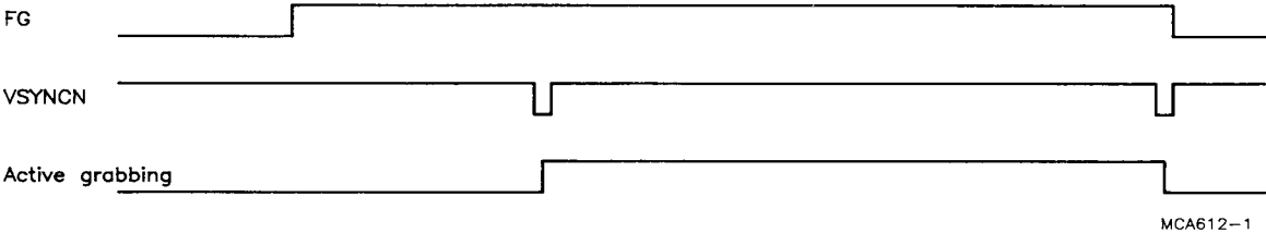
Fig.17 Frame Grabbing in the non-interlace, double frequency and interlace field repeat modes.
