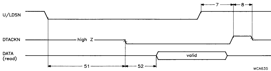
Fig.40 Internal register access.
