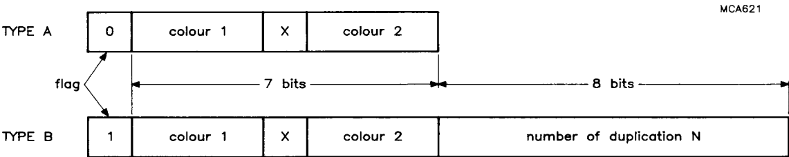
Fig.23 Run-length format in 4 bits/pixel.
