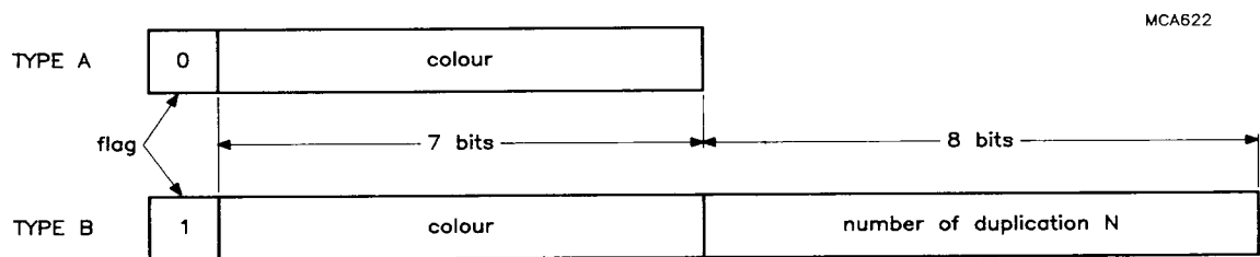
Fig.21 Run-length format in 8 bits/pixel
