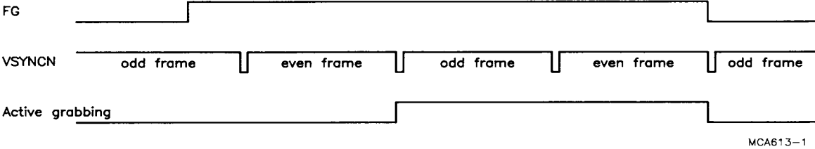
Fig.18 Frame Grabbing in the interlace mode.
