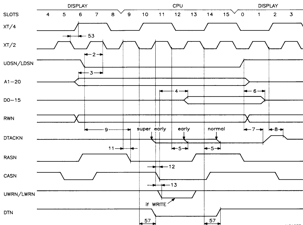
Fig.42 CPU &lt;-&gt; memory access in FAST mode.
