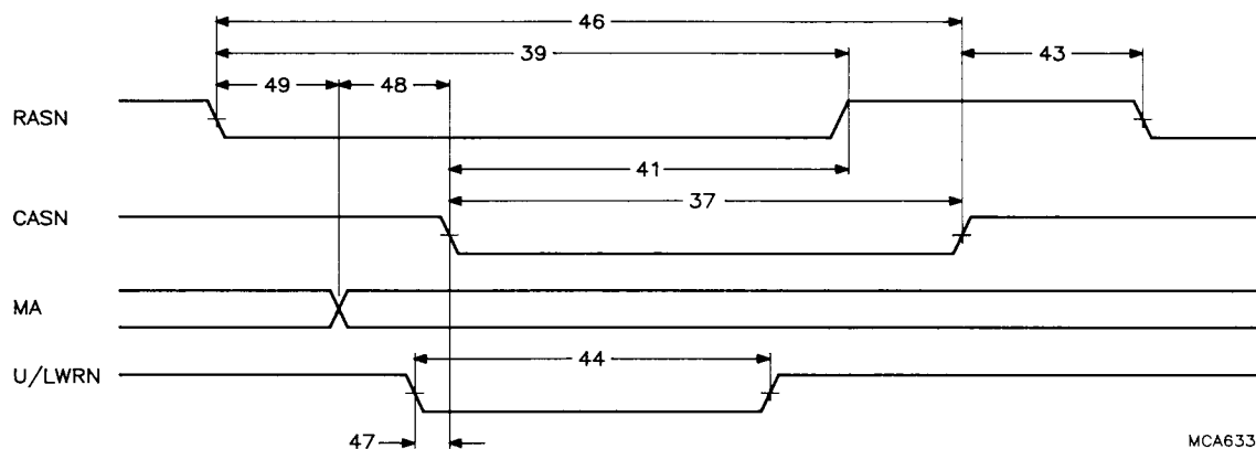
Fig.38 Signals in CPU window.
