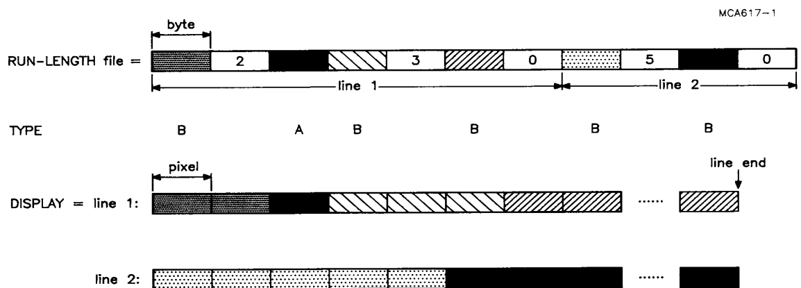
Fig.22 Run-length file display, 8 bits/pixel.
