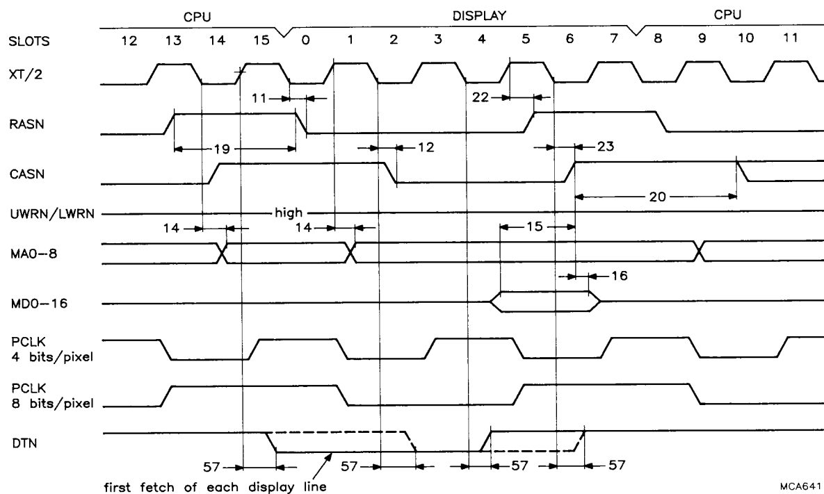
Fig.45 Display cycle in NORMAL mode.
