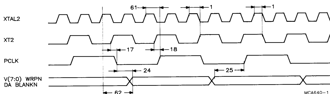
Fig.46 Pixel output timing.
