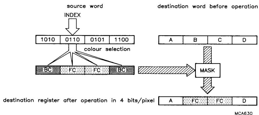
Fig.30 BCOLOUR1 example.
