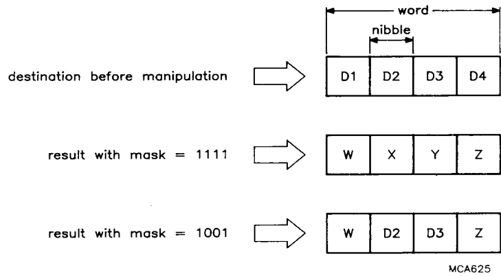
Fig.36 Mask example.
