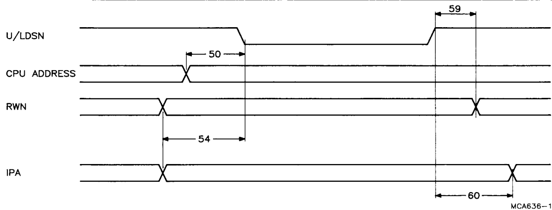
Fig.41 CPU access.
