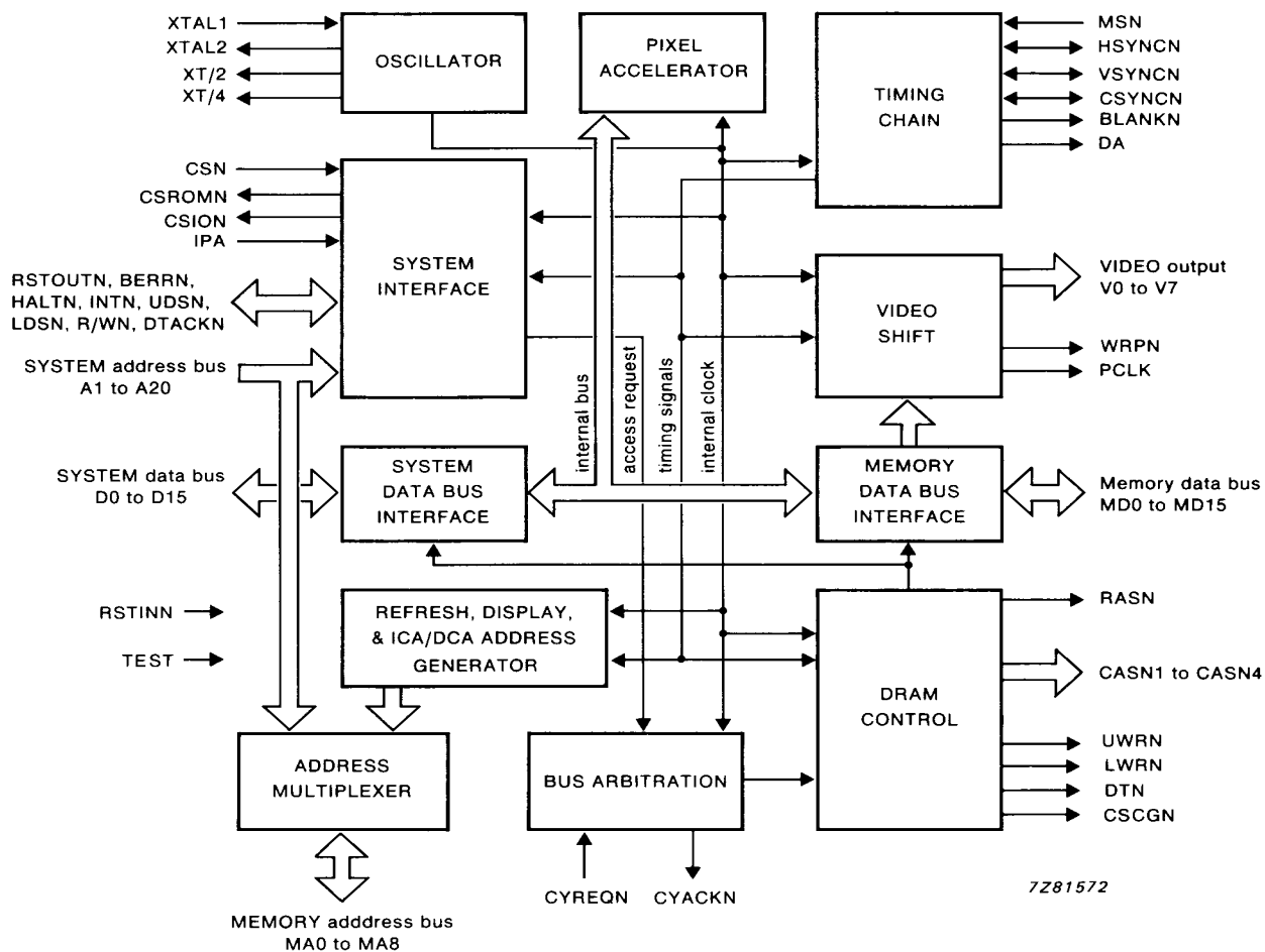
Fig.1 Block diagram.
