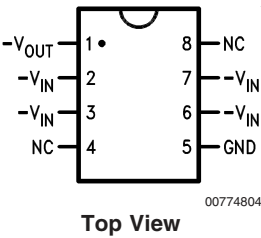
SO-8 Plastic (Narrow Body)
