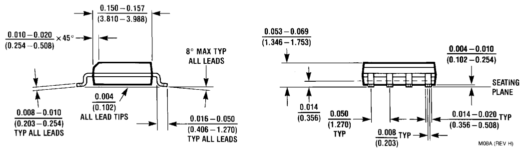
SOIC Package (M) NS Package Number M08A
