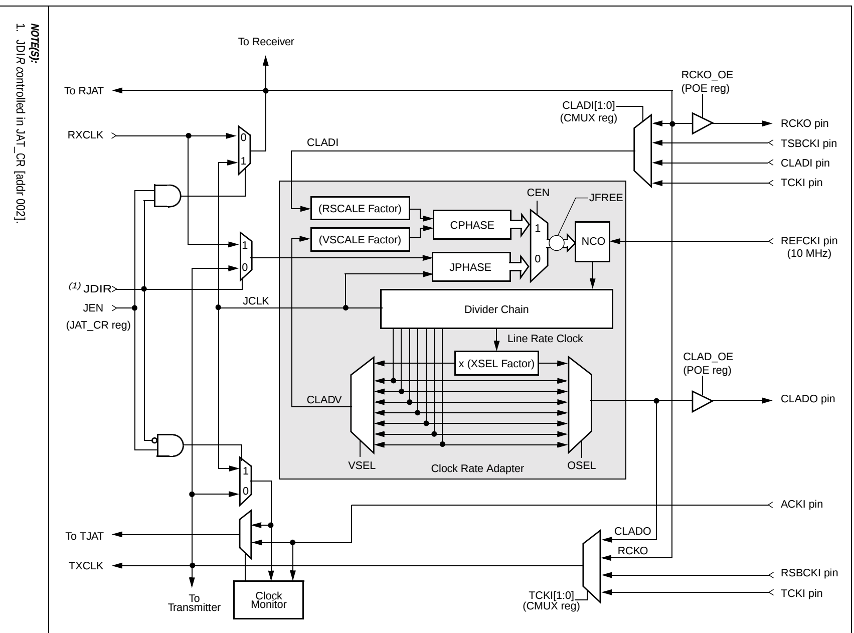
Figure 2-21. Clock Rate Adapter/Jitter Attenuator Block Diagram (Bt8370 and Bt8375 Devices)
