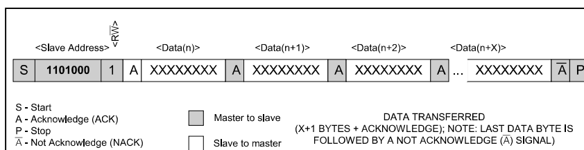
Figure 5. Data Read—Slave Transmitter Mode
