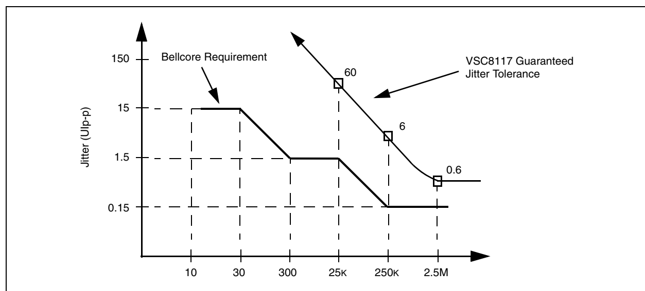
Figure 7. Jitter Tolerance
