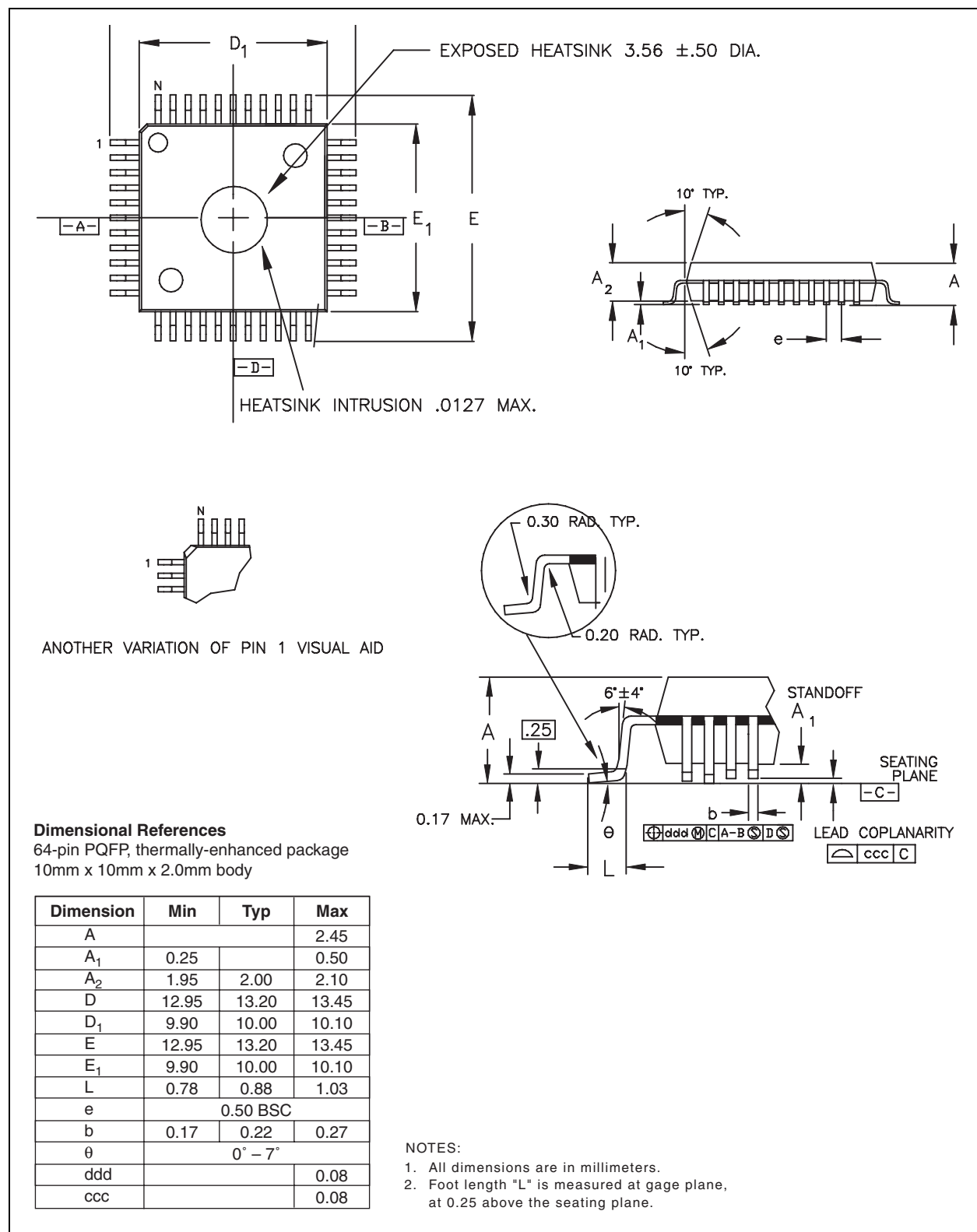
Figure 13. Package Drawing
