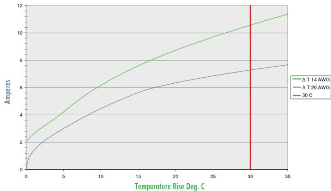
Figure 2. Temperature Rise vs. Current
