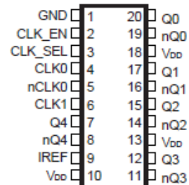
85105I 20-Lead TSSOP 6.5mm x 4.4mm x 0.925mm Package Body G Package Top View
