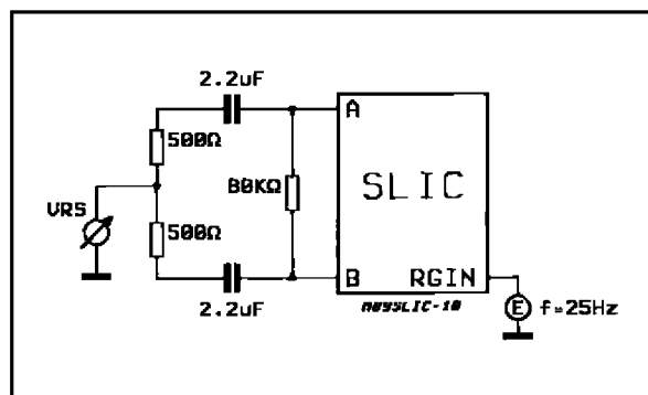
Figure 10 : Ringing Symmetry.
