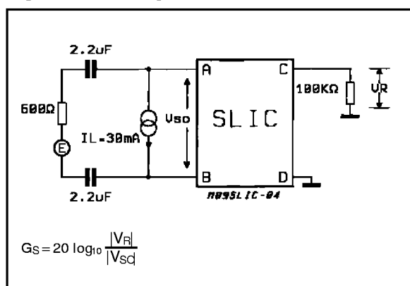
Figure 4 : Sending Gain.
