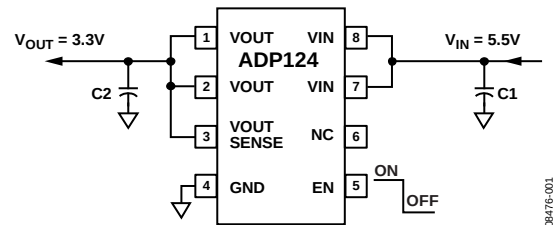
Figure 1. ADP124 with Fixed Output Voltage
