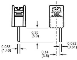
04 Wire Wrap Tail
