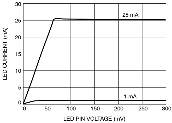
Figure 9. Dropout Characteristics
