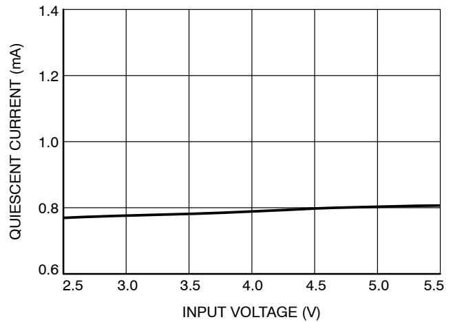
Figure 4. Quiescent Current vs. Input Voltage (Full Load)
