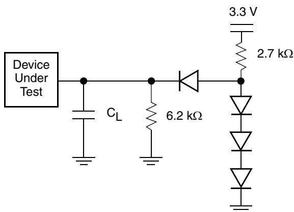
Figure 16.1 Test Setup
