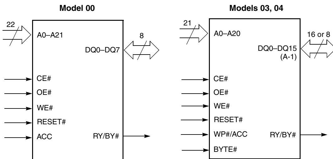
Figure 5.1 Logic Symbols
