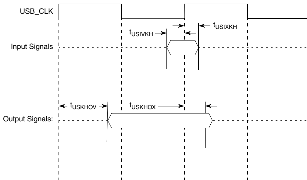
Figure 20. USB signals
