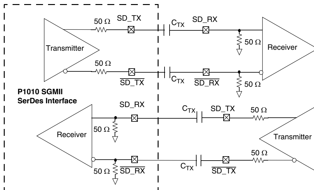
Figure 12. 4-Wire AC-coupled SGMII serial link connection example
