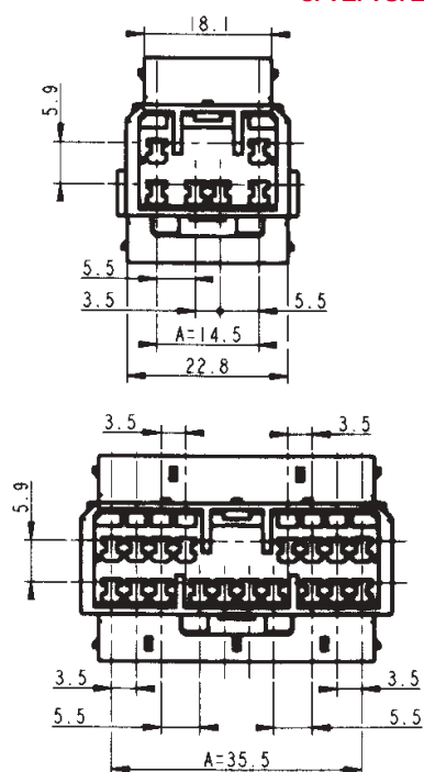
6/12/18/20 way male housings
