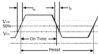
Figure 7. Output Waveform
