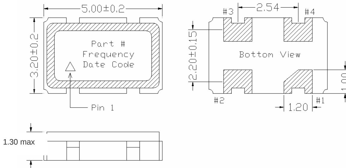
Figure 9, Package drawing
