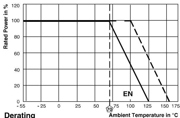
Derating
