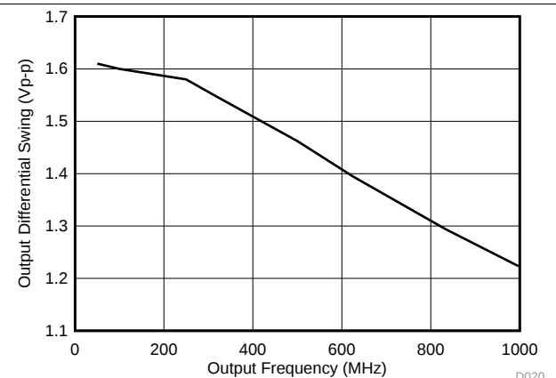
Figure 18. AC-LVPECL Differential Output Swing vs Frequency
