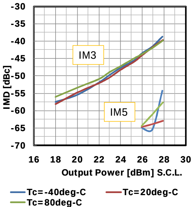
IMD Performance vs. Output Power by Temperature V_{DS}=10V @7.2GHz
