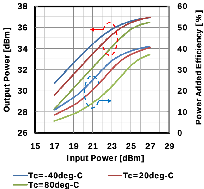
Input Power vs. Output Power, Power Added Efficiency by Temperature V_{DS}=10V @7.2GHz
