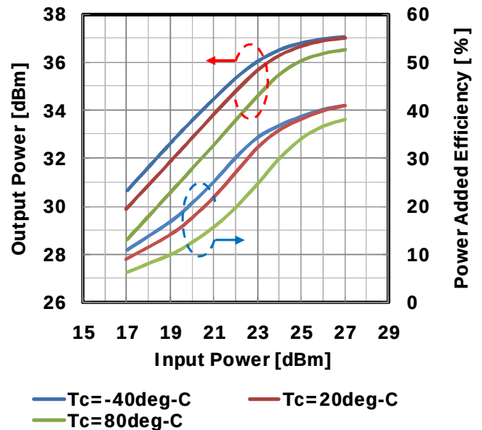
Input Power vs. Output Power, Power Added Efficiency by Temperature V_{DS}=10V @6.8GHz
