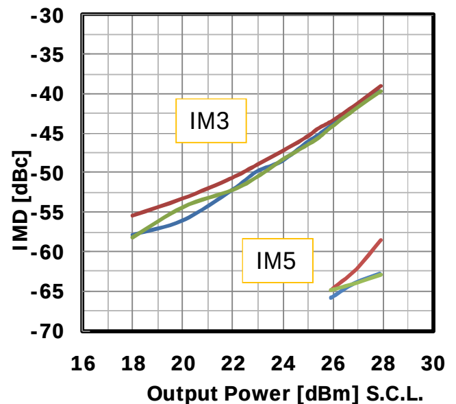
IMD vs. Output Power
